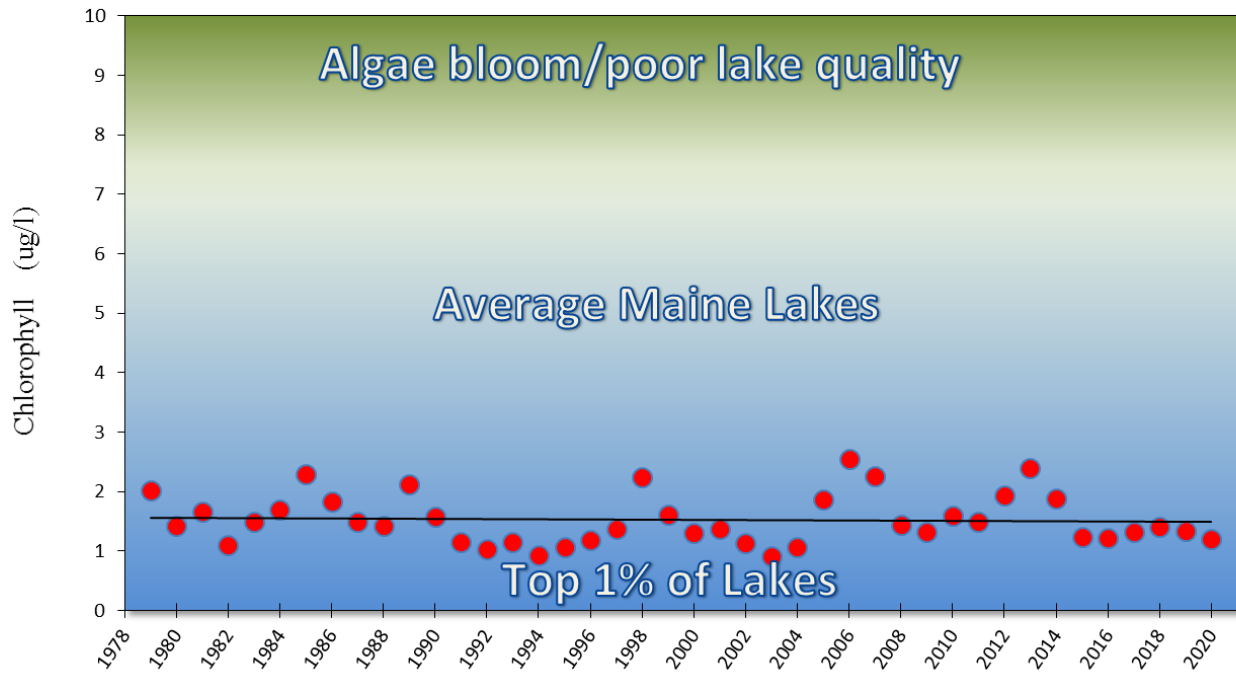
Sebago Lake Yearly Average Lower Bay Chlorophyll
